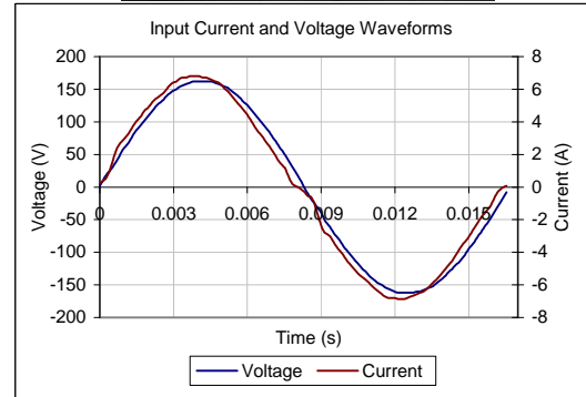
Input AC Current Waveform (ITHD = 9.14%, 50% Load)
