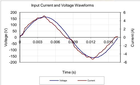
Input AC Current Waveform (ITHD = 16.55%, 50% Load)
