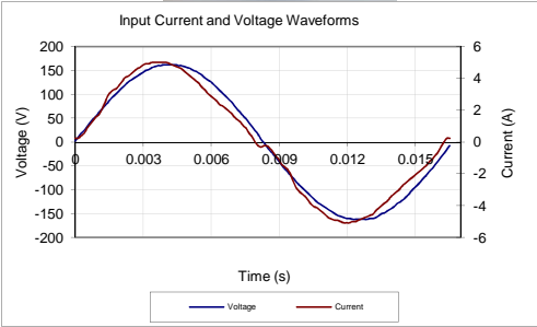
Input AC Current Waveform (ITHD = 8.93%, 50% Load)
